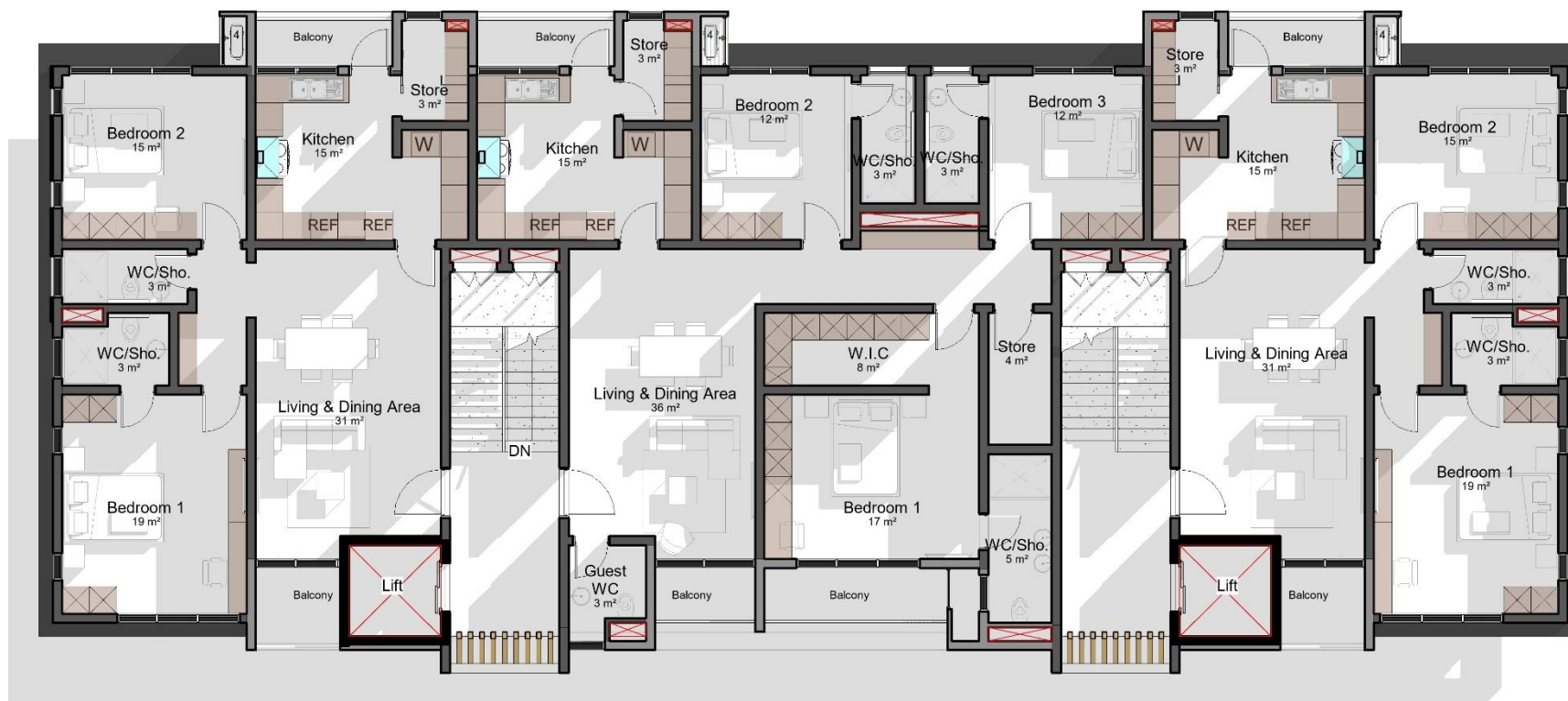
1 ST FLOOR PLAN - 382 sqm
