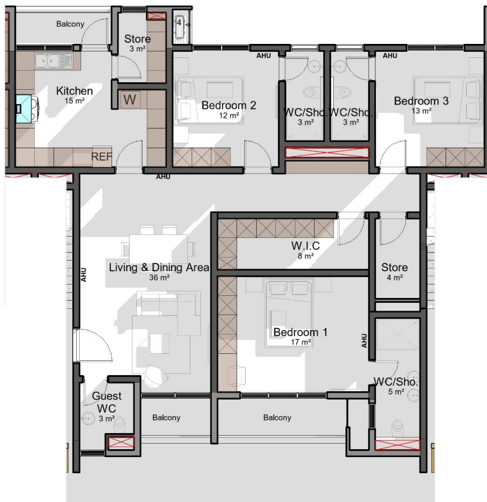
3 BEDROOM APARTMENT- 150 sqm
